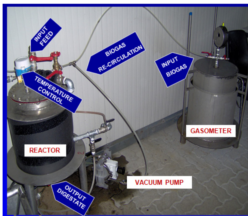
Figure 1 The pilot hardware description is illustrated. The same reactor, in different six-month fermentation sessions, with two different pre-treated feedings was used during this research study.
