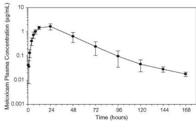
Fig. 2B. Plasma meloxicam concentration (mean \pm SEM) meloxicam with gabapentin treatments in calves. Pharmacokinetic parameter estimates
