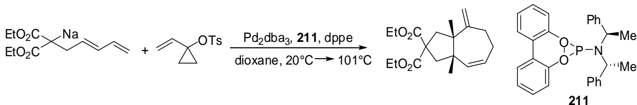
Scheme 92. One-pot Pd-catalyzed coupling-cycloaddition
