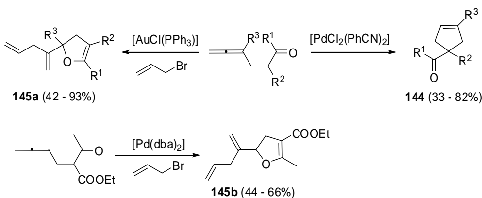
Scheme 55. Preparation of cyclopentenes and 4,5-dihydrofurans from 2-(2',3'-allenyl)acetylacetates
