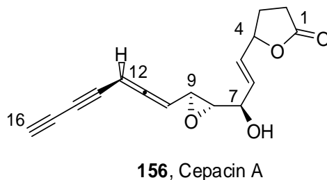
Figure 3. Cepacin A structure
