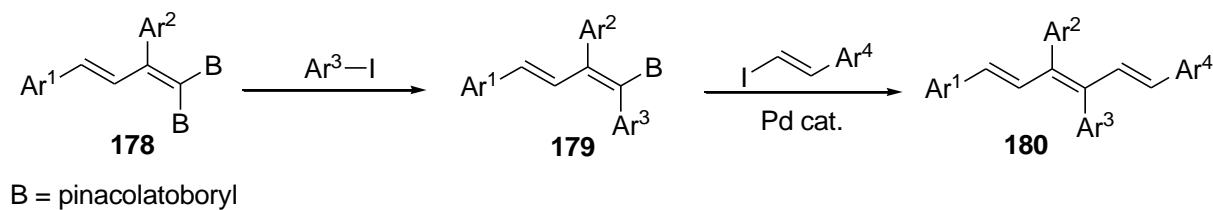
Scheme 73. Synthesis of 1,3,4,6-tetraarylated 1,3,5-hexatrienes
