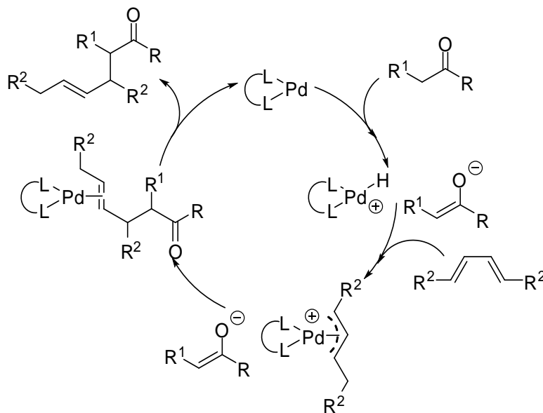
Scheme 89. Mechanism of the palladium-catalyzed addition of the \alpha -C-H to conjugated dienes
