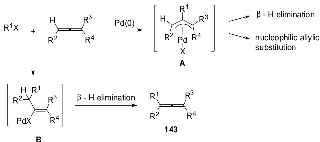
Scheme 54. Proposed mechanism for 1,2-allenyl sulfones arylation
