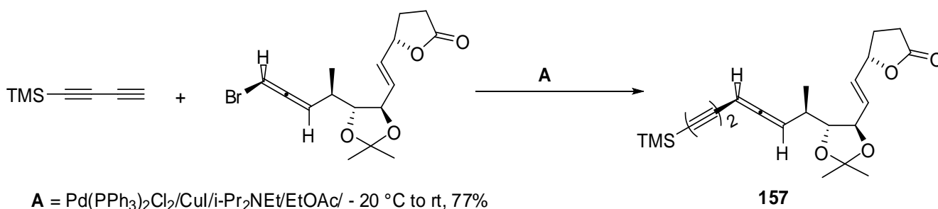
Scheme 62. Diyne moiety coupling onto the allenic fragment
