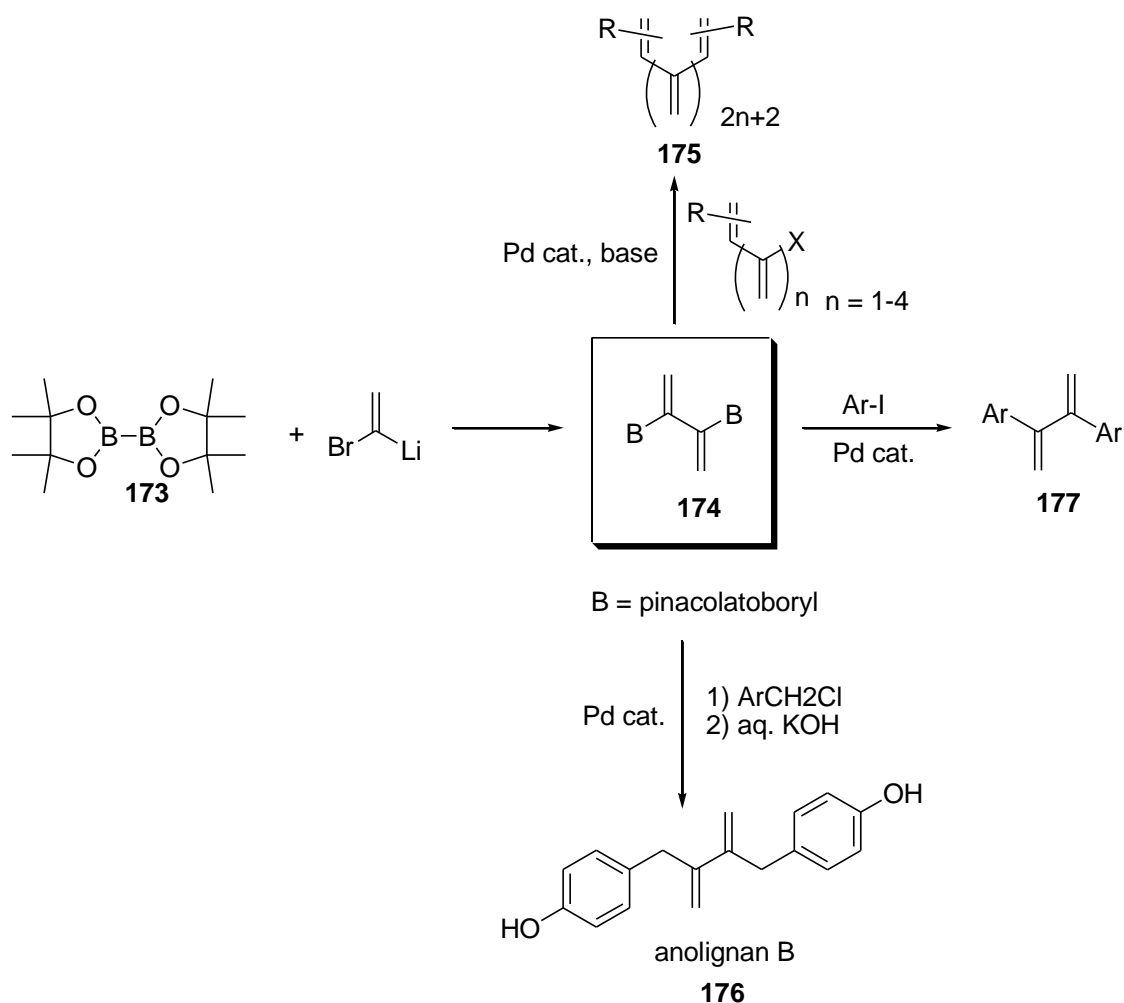
Scheme 72. Palladium-catalyzed coupling of 2,3-bis(pinacolato)boryl-1,3-butadiene with organic halides
